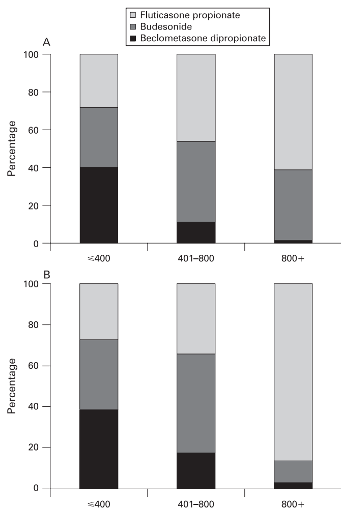
Figure 3 Percentages of asthmatic children aged under 5 (A) and aged 5 to under 12 years (B) prescribed inhaled corticosteroids by steroid and dose (<400, 400–800 and 800+ µg/day) between 1992 and 2004.
